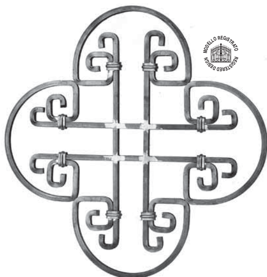
Art. 1028/2 12 x 12 mm Ø 630 mm
