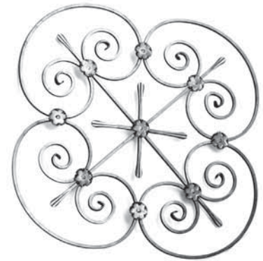
Art. 26/B/2 ∅ 10 x 10 mm H 810 mm L 810 mm
