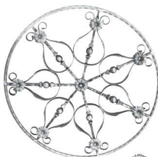
Art. 718/1 ∅ 14 x 14 mm ∅ 735 mm
